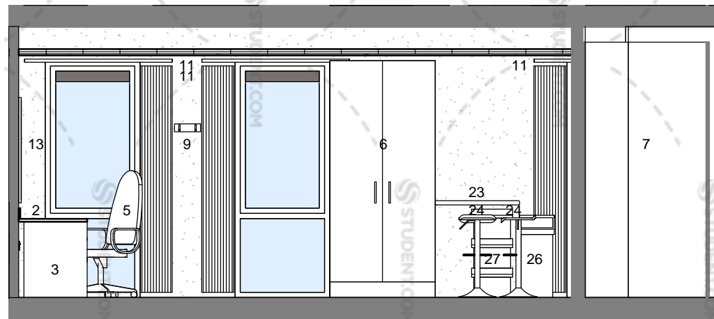
PB6 Elevation 2 1 : 50
