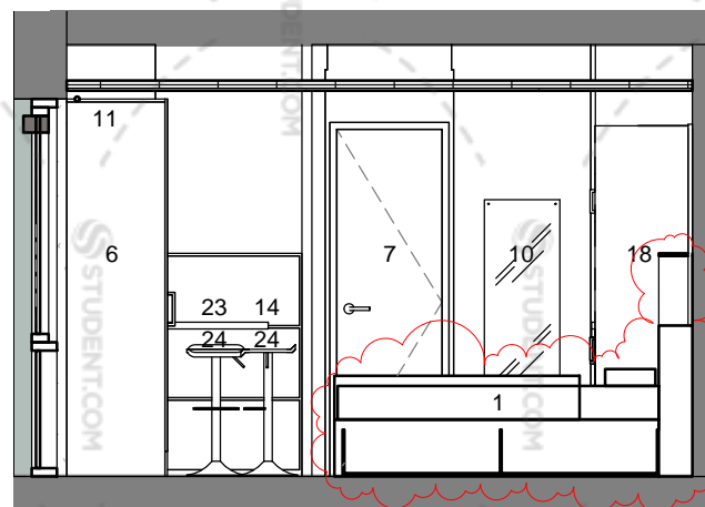
PB6 Elevation 3 1 : 50
