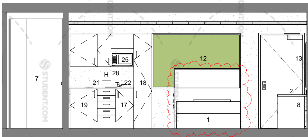
PB6 Elevation 4 1 : 50
